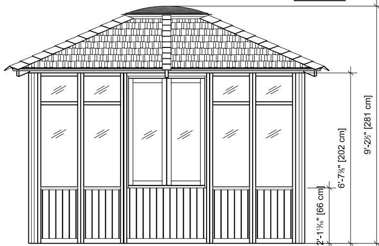
Side Elevation
